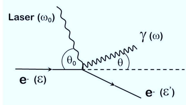
Figure 1: Compton scattering schematics.
