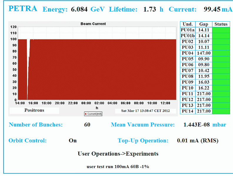
Figure 4: PETRA online status display [26].
