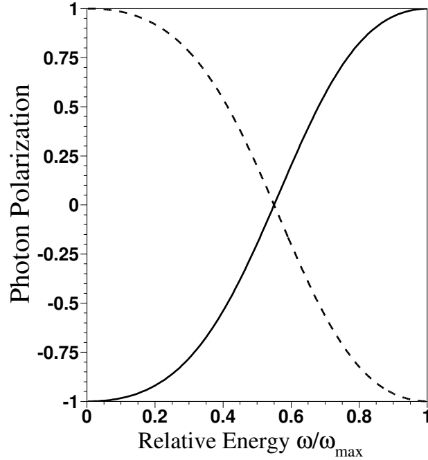
Figure 2: Polarization of the Compton scattered photon on a 6 GeV electron as a function of the photon energy. The solid and dotted lines correspond to the initial laser light helicity: +1 solid, -1 dotted.
